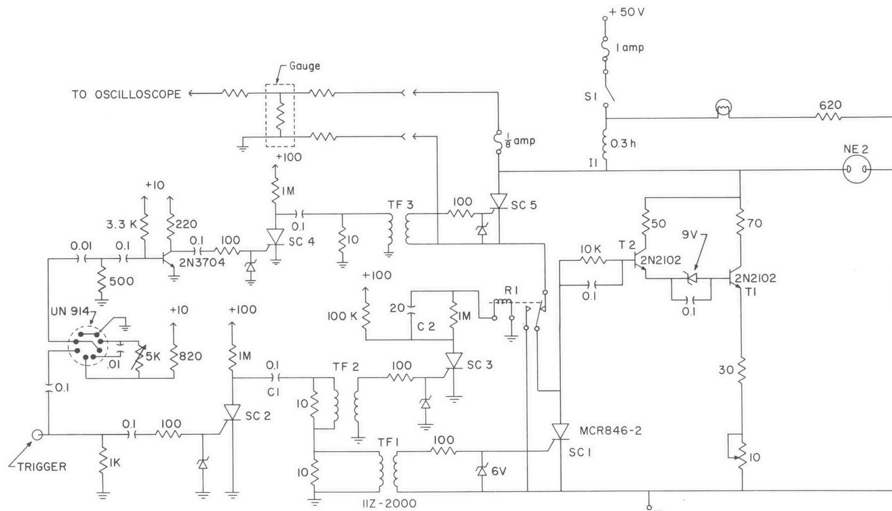
Fig. 22. Schematic of manganin gauge constant current supply.
